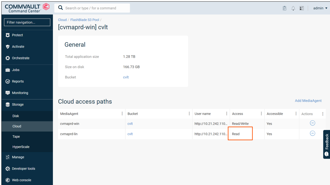
Figure 3. Cloud storage target access paths.
